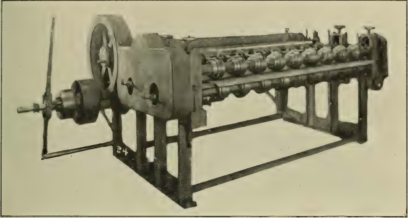
FIG. 135.—Shingle Cutter—Front View.
